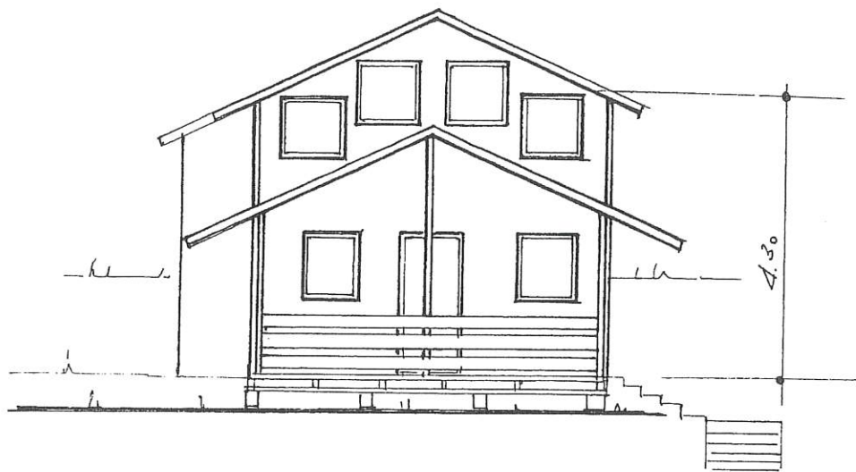
NORTH-WEST VIEW
